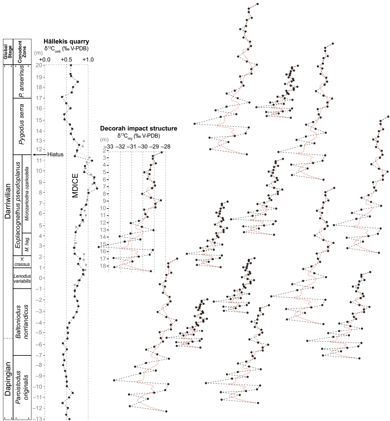
Fig. 1. \delta^{13}\text{C}_{\text{carb}} chemostratigraphy at the Hällekis quarry, modified from Schmitz et al. (2010; Dapingian added according to Bergström et al. 2009), with grey points indicating the data as reproduced by Bergström et al. (2009, fig. 4). To the right, a selection of potential fits of the Winneshiek Shale \delta^{13}\text{C}_{\text{org}} data (Bergström et al. 2009) against the Hällekis data are indicated, in order to illustrate the many arbitrary scenarios possible when assessing the age of the Winneshiek Shale succession based merely on visual comparison of \delta^{13}\text{C} records (note: we do not propose any of these scenarios to be correct). The leftmost version represents the approximate scenario preferred by Bergström et al. (2009). Note the extreme difference in the amplitude of \delta^{13}\text{C} variability between the Winneshiek and Hällekis data sets, and that these simple 'age models' do not take into account potential problems of correlating \delta^{13}\text{C}_{\text{org}} with \delta^{13}\text{C}_{\text{carb}} locally, regionally and globally (see main text). [Colour figure can be viewed at wileyonlinelibrary.com ]
